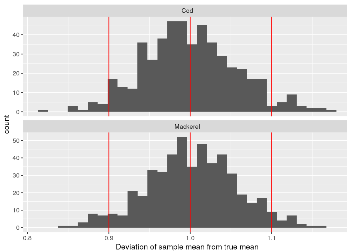
Figure 10. Deviation of the sample mean for the true mean.
