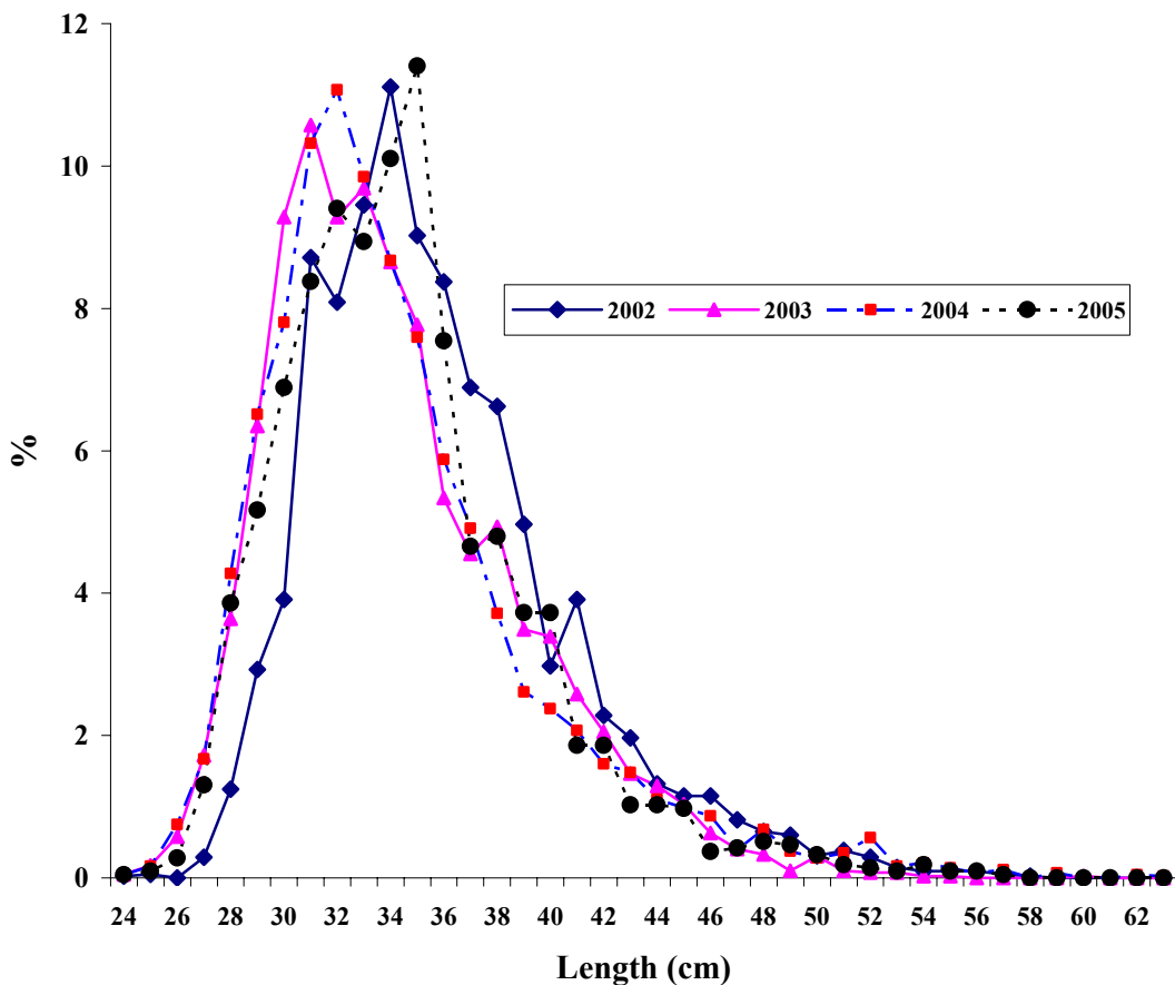
Figure 20: Length distribution of L. mahsena in the catch of Saya de Malha bank for the period 2002-2005.
