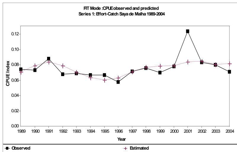
Figure 10: Observed and predicted values of CPUE on Saya de Malha bank using the dynamic non-equilibrium Logistic model in ASPIC for the period 1989-2004.
