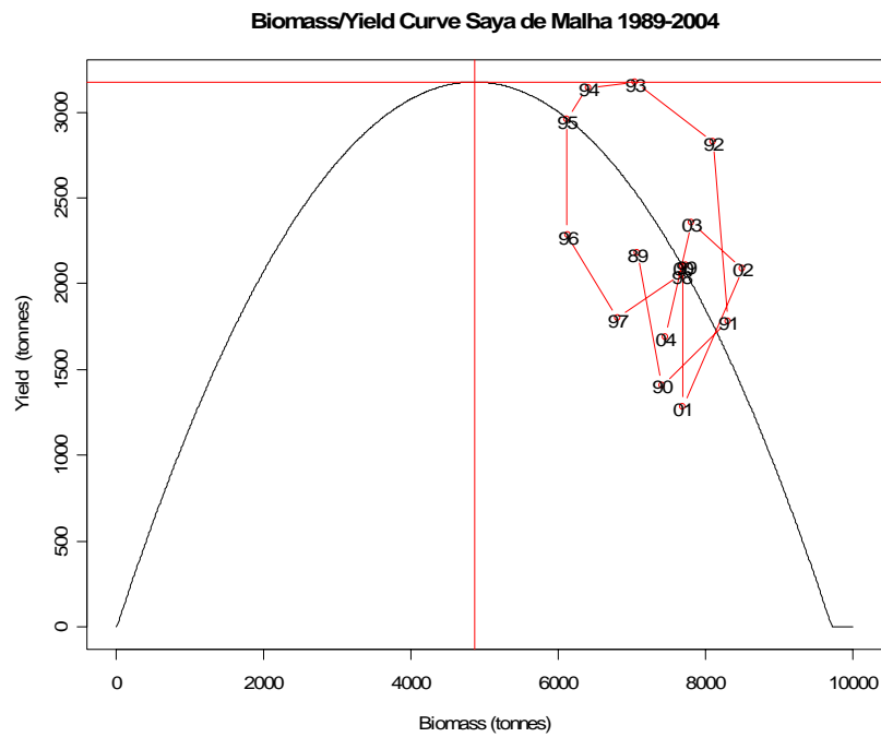
Figure 7: Biomass and yield curve showing observed and predicted yield trajectory on Saya de Malha bank for the period 1989-2004.
