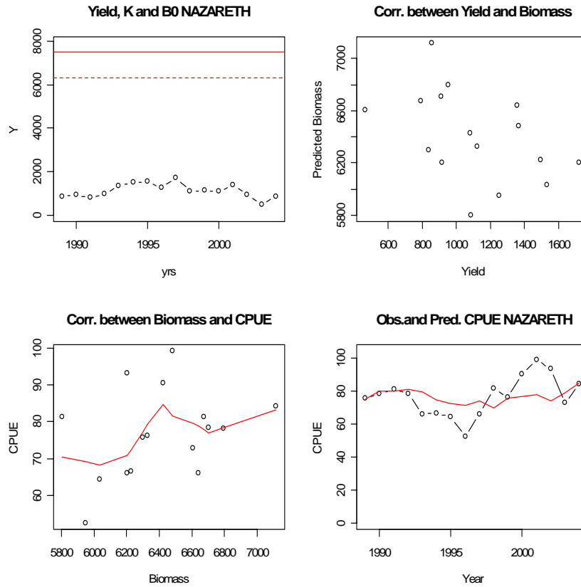
Figure 8: Correlation of yield, K , B_t , CPUE, observed and predicted CPUE for Nazareth bank using the non-equilibrium dynamic biomass model.
