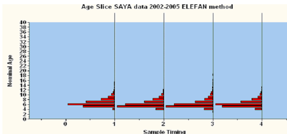
Figure 22 : VBGF fitted on the length frequency distribution of L. mahsena (2002) using the ELEFAN method in LFDA (a) and age slice of length frequency data (2002-2005) from Saya de Malha bank (b).
