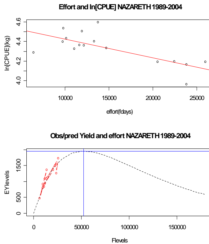
Figure 5: Effort, CPUE, observed and predicted yield on Saya de Malha bank (a) and Nazareth bank (b) using the FOX equilibrium assumption model.
