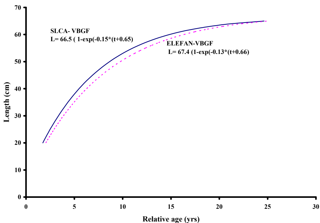
Figure 23 : VBGF curves of L. mahsena length frequency from Saya de Malha bank (2002-2005) fitted using the SLCA and the ELEFAN methods.
