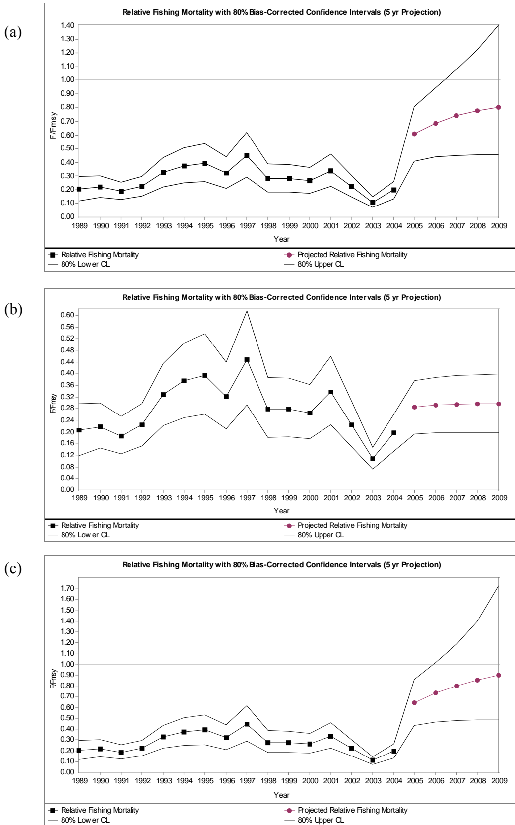
Figure 19: Five year projection (2005 to 2009) trajectories of relative fishing mortality ( F/F_{MSY} ) with annual catch at the estimated MSY level of 2,377 t (a), annual catch at 1,200 t (b) and annual catch at 2,500 t (c) on Nazareth bank.
