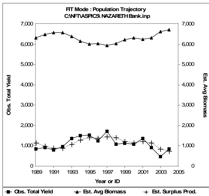
Figure 16: Observed yield, estimated surplus production and average biomass on Nazareth bank using the Logistic model in ASPIC 5 for the period 1989-2004.
