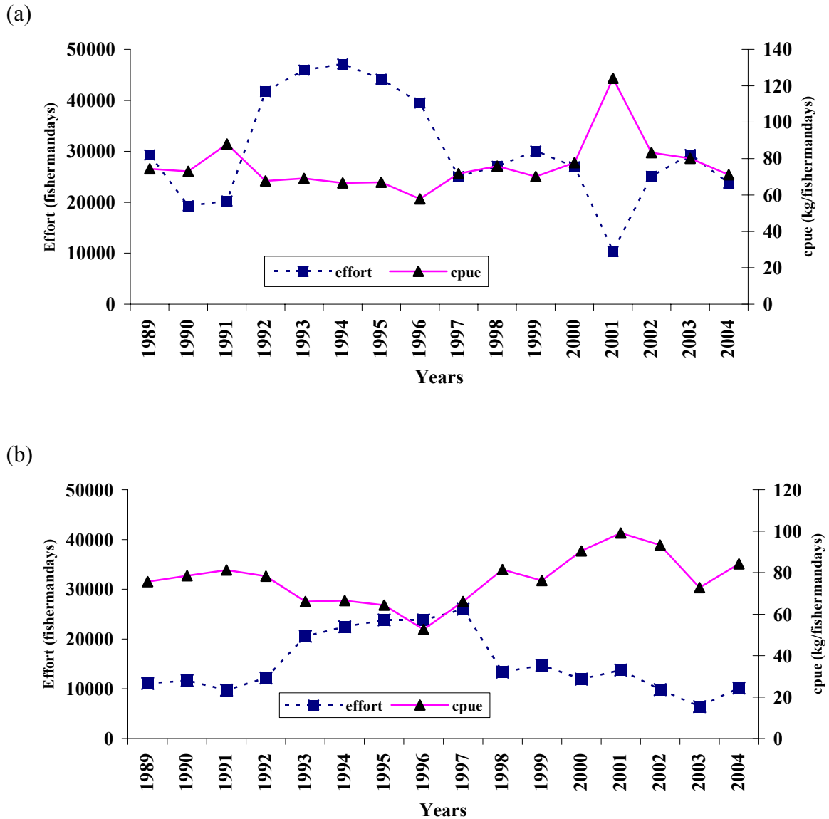
Figure 3: Effort and CPUE trends on Saya de Malha bank (a) and Nazareth bank (b) for the period 1989-2004.
