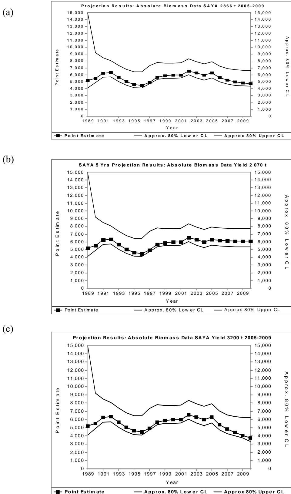
Figure 12 : Five years projection (2005 to 2009) trajectories of absolute biomass with annual catch at the MSY level of 2,886 t (a), annual catch at 2,070 t (b) and annual catch at 3,200 t (c) on Saya de Malha bank.
