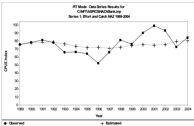
Figure 15: Observed and predicted values of the CPUE index on the Nazareth bank using the non-equilibrium Logistic model in ASPIC.
