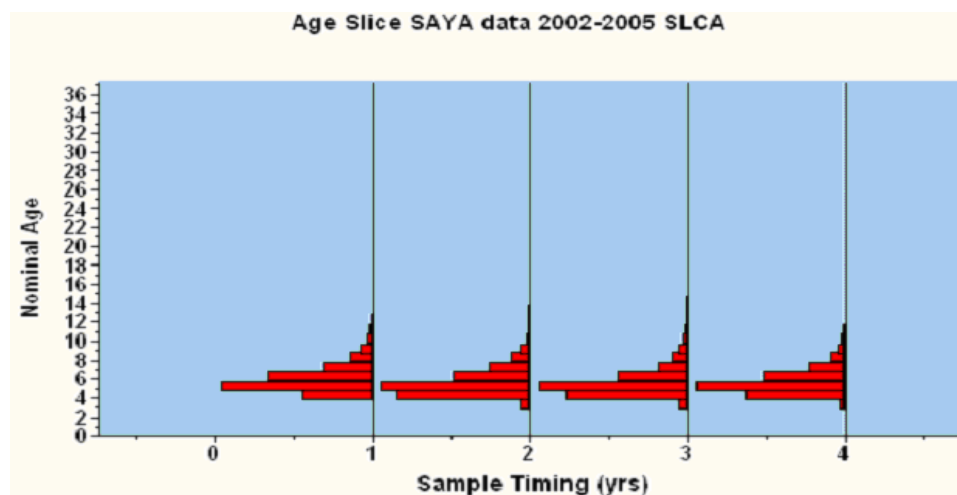
Figure 21: VBGF fitted on the length frequency distribution of L. mahsena (2002) using the SLCA method in LFDA (a) and age slice of length frequency data (2002-2005) from Saya de Malha bank (b).
