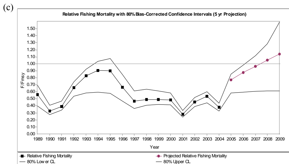
Figure 14: Five year projection (2005 to 2009) trajectories of relative fishing mortality ( F/F_{MSY} ) with annual catch at the MSY level of 2,886 t (a), annual catch at 2,070 t (b) and annual catch at 3,200 t (c) on Saya de Malha bank.
