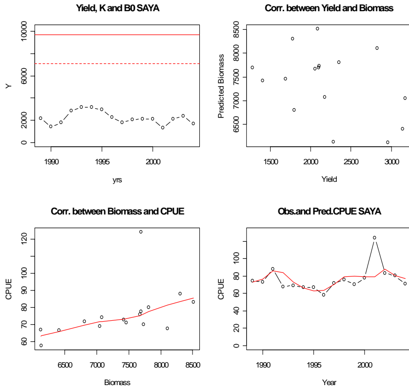
Figure 6: Correlation of yield, K , B_t , CPUE, observed and predicted CPUE for Saya de Malha bank using the non-equilibrium dynamic biomass model.
