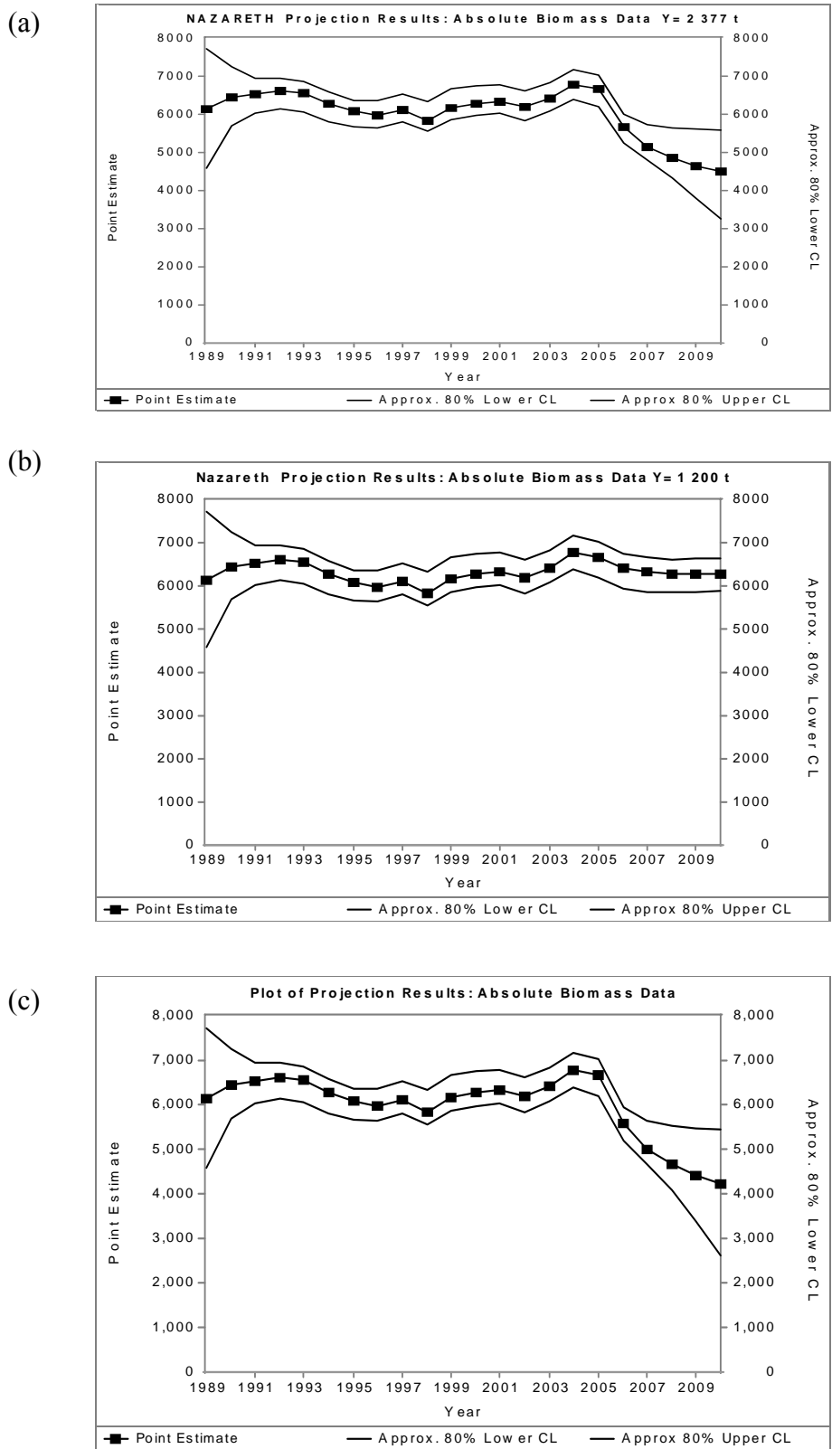
Figure 17: Five year projection (2005 to 2009) trajectories of absolute biomass with annual catch at the estimated MSY level of 2,377 t (a), annual catch at 1,200 t (b) and annual catch at 2,500 t (c) on Nazareth bank.
